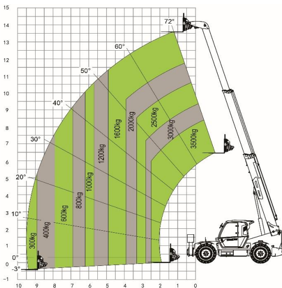
Without stabilizer
