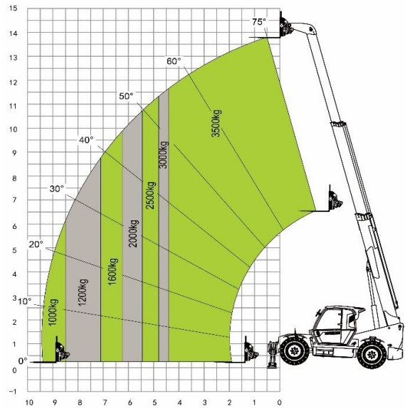
With stabilizer
